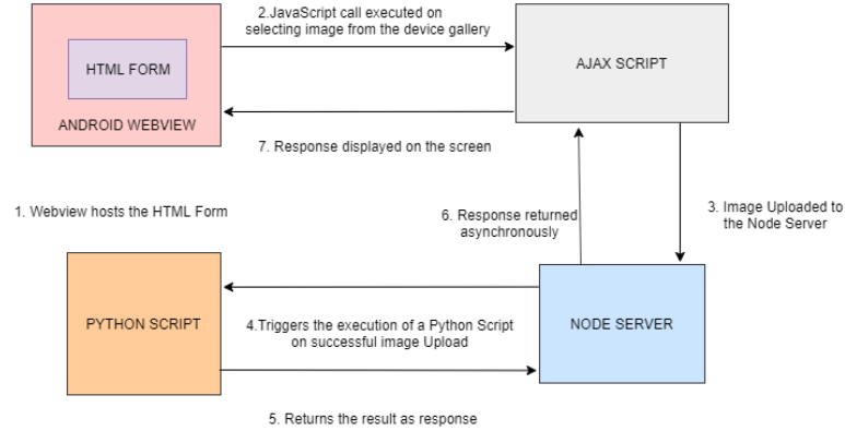
Figure 1: System design
