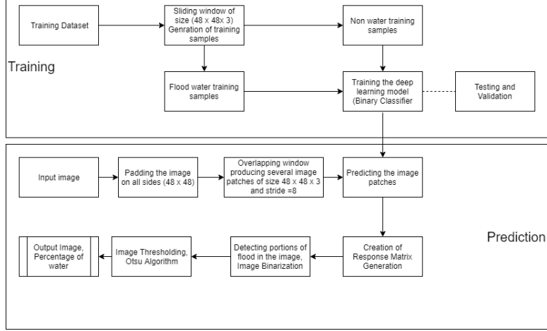
Figure 5: Flowchart
