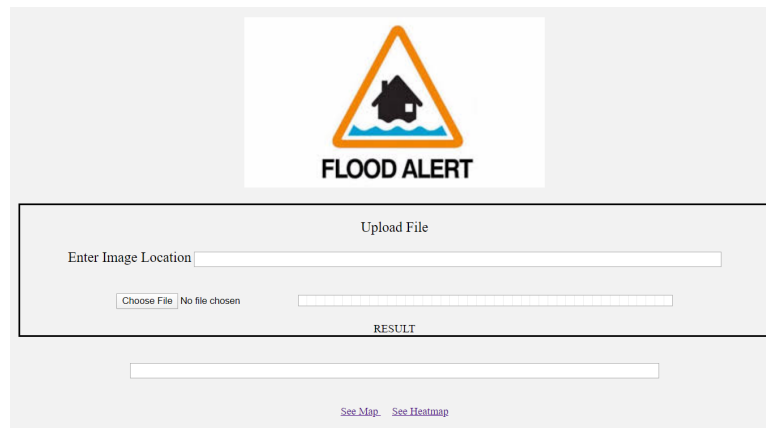
Figure 3: UI design
